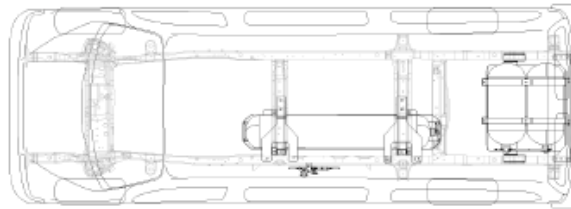
E-230/350 Van – 20GGE = 17.6 DGE
